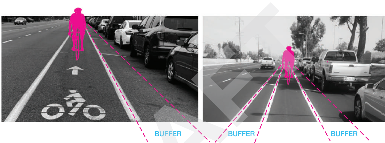
(Left) Buffered Bike Lane on the Parking Side - Moreno Valley, CA
