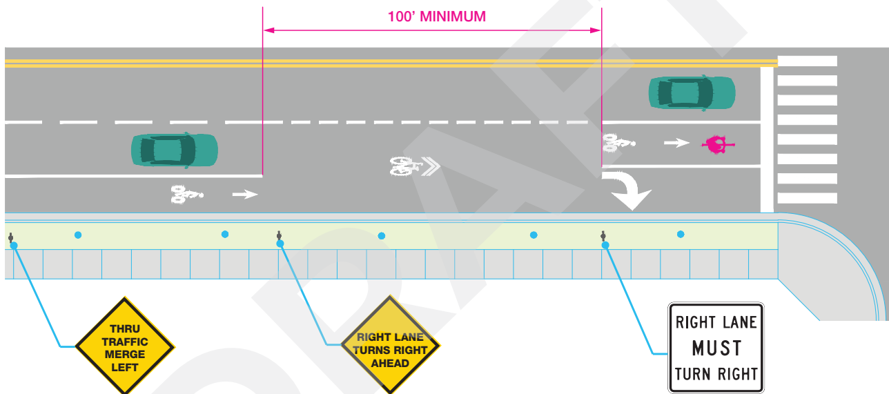
Additional Signage as Length of Turn Lane Increase
