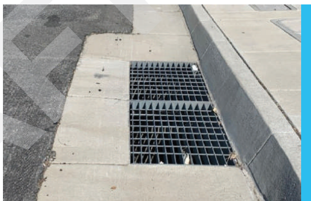
Bicycle-Friendly Drainage Grate
