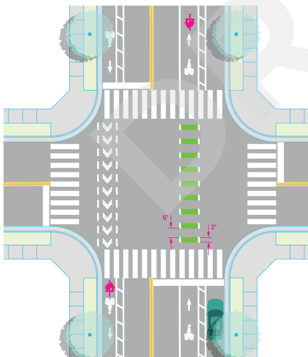
Bicycle Pavement Markings Through Intersections
