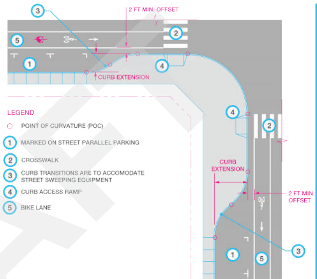
Example of a Curb Extension (Bulb Out)
