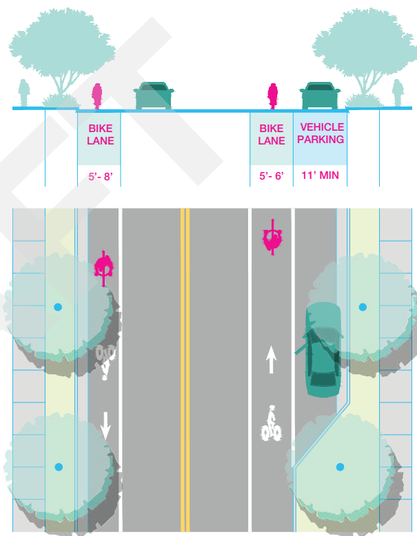
Typical Dimensions of Bike Lanes
